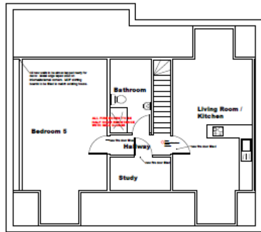
Proposed Loft Floor Plan
